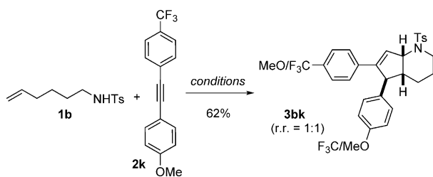
Scheme 2. An unsymmetrical alkyne.
